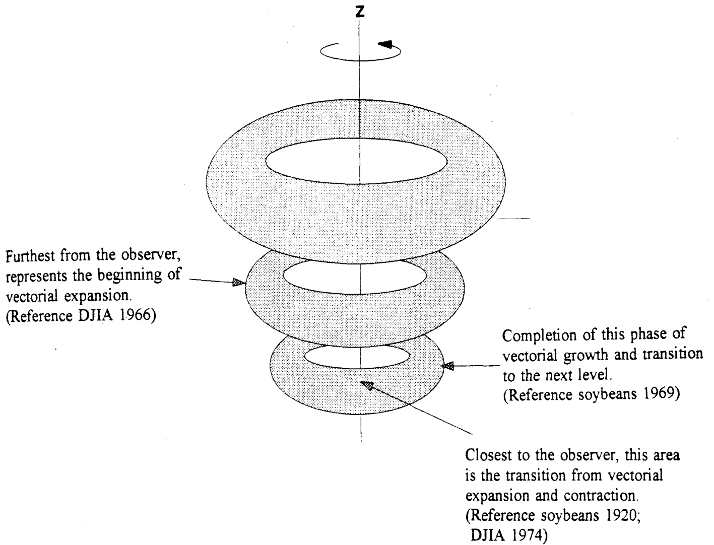
Figure 13.9 Tori Increase In Size With Increasing Energy Levels
