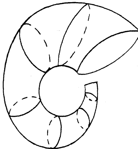
Figure 13.3 A Curved Tunnel Forms A Nautilus Shell
