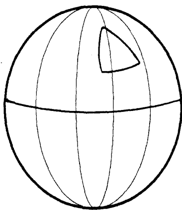
Figure 13.7 The Sum Of The Three Inner Angles Of A Triangle On The Surface Of A Sphere Is Greater Than 180^\circ
