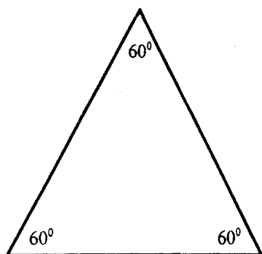
Figure 13.5 Sum Of The Three Inner Angles Of A Triangle On A Plane Is 180^\circ
