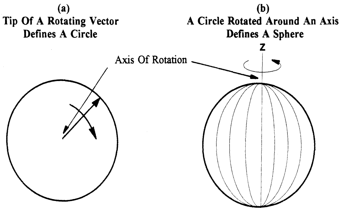
Figure 13.1 Rotation Of A Vector; (a) Around A Single Axis; (b) Around Two Orthogonal Axes
